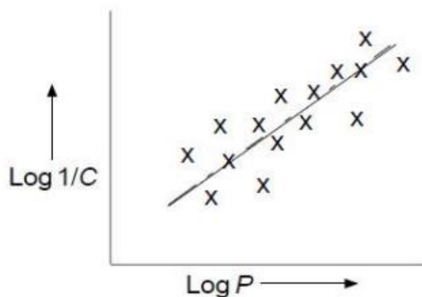
Fig.10 Regression analysis
