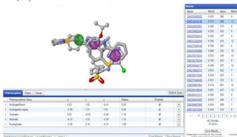
Fig.9 Virtual screening
