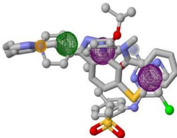
Fig.8 Pharmacophoric features
