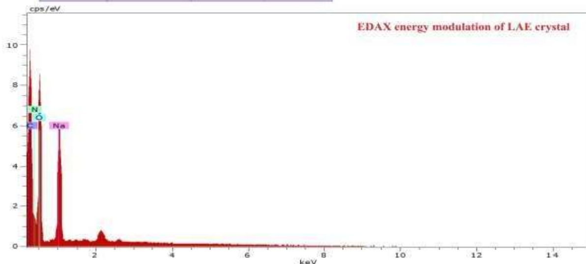
Figure 4: EDAX examination spectrum
