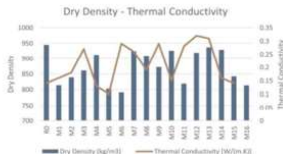
Fig. 9. Dry density (kg/m 3 ) vs. thermal conductivity [W/(m.k)]
