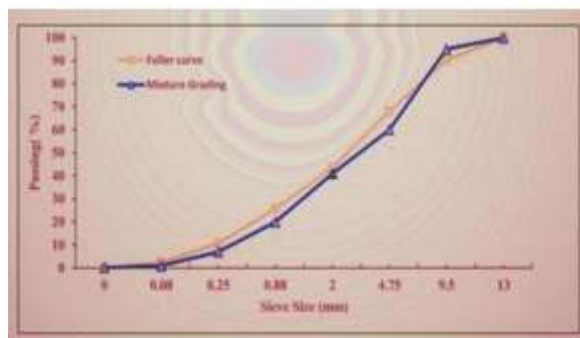
Fig 2. Fuller curve and aggregate gradation
