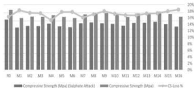
Fig. 7. Compressive Strength Loss after sulphate attack at 180 days.
