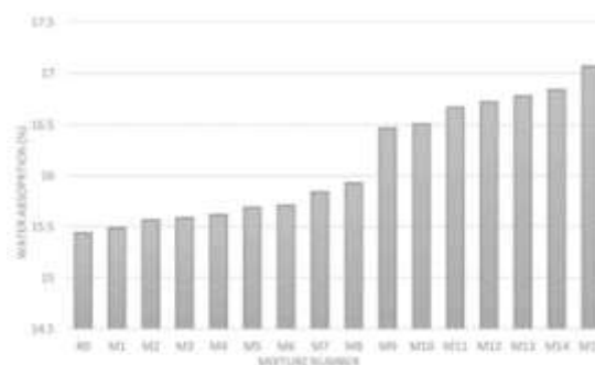
Fig.13. Water absorption
