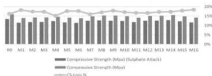
Fig. 5. Compressive Strength Loss after sulphate attack at 28 days.
