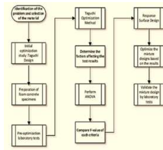
Fig 1. Exploration flow-chart
