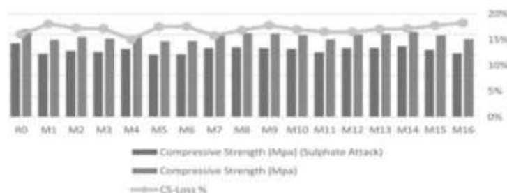
Fig. 4. Compressive Strength Loss after sulphate attack at seven days.
