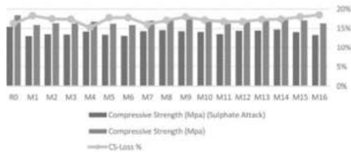
Fig. 6. Compressive Strength Loss after sulphate attack at 90 days.
