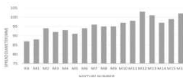
Fig. 11. Spread Test Diameter
