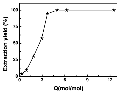
Figure 1. Extraction yield of UO_2^{2+} by 3f as a function of Q . V_{\text{org}} = 5.0 mL, [Ex.] = 1.0 mmol L^{-1} , V_{\text{aq}} = 5 mL, pH^i = 0.6 , t = 30 min, T = 22 °C.
