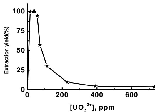
Figure 2. UO_2^{2+} extraction yield versus initial molar UO_2^{2+} concentration. V_{\text{org}} = 5.0 mL, [Ex.] = 1.0 mmol L^{-1} , V_{\text{aq}} = 5.0 mL, pH_i = 0.65 , t = 30 min, T = 22 °C
