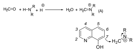
Scheme 3: Mechanism (A).
