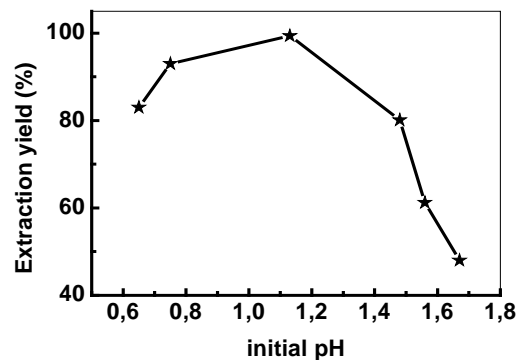
Figure 3. pH effect on the extraction of UO_2^{2+} . V_{\text{org}} = 5.0 mL, [Ex.] = 1.0 mmol L^{-1} , V_{\text{aq}} = 5 mL, [UO_2^{2+}]_{\text{initial}} = 60 ppm, t = 30 min, T = 22 °C
