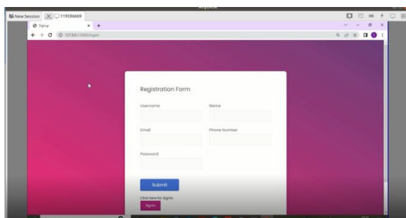
Fig.4: User registration
