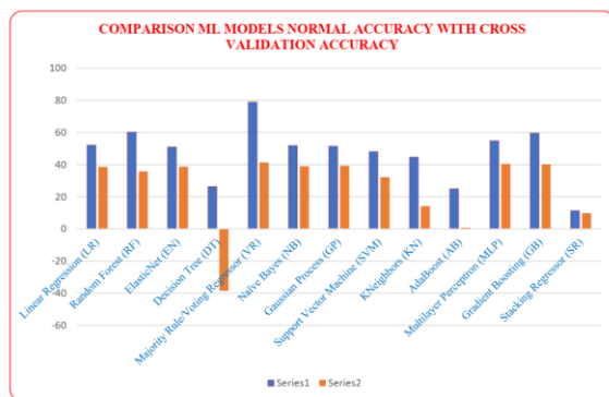
Fig:4 Comparison ML Models Normal Accuracy with Cross Validation Accuracy
