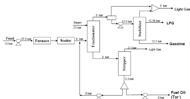
Figure 1. Block flow diagram of visbreaking process
