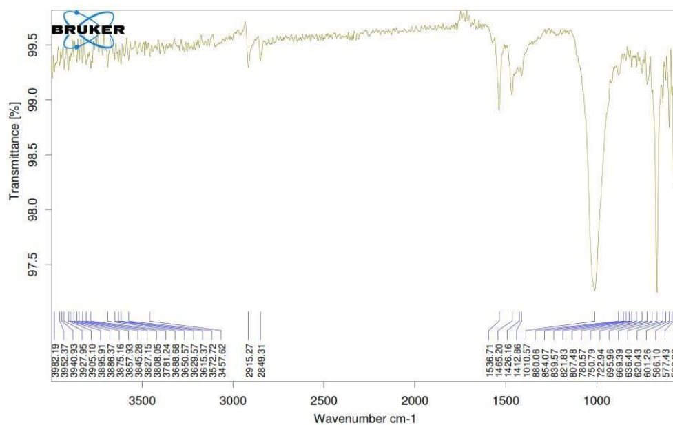
Figure No.1: FT-IR of Pioglitazone Pure Drug
