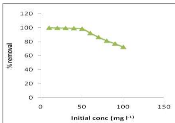
Fig. 12: The percentage removal of Chromium(VI) as the concentration of Chromium(VI) ion solution
