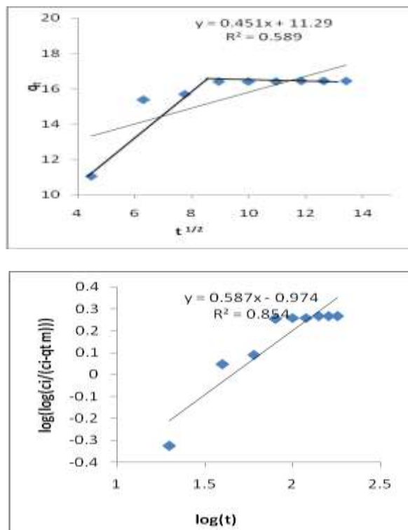
Fig. 15: Model of Elovich, diffusion of weber and Morris intra particle, Pseudo first-order reaction Bang ham's pore diffusion, Pseudo second-order
