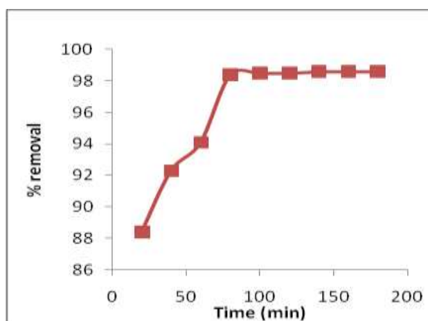
Fig. 11: The percentage removal of Chromium(VI) as a contact time (min)
