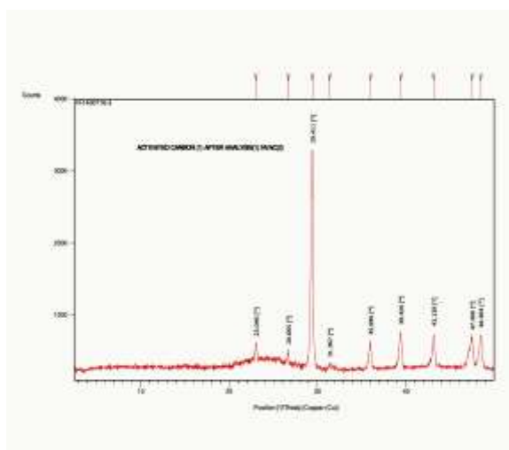
Fig. 6: After Analysis Of XRD
