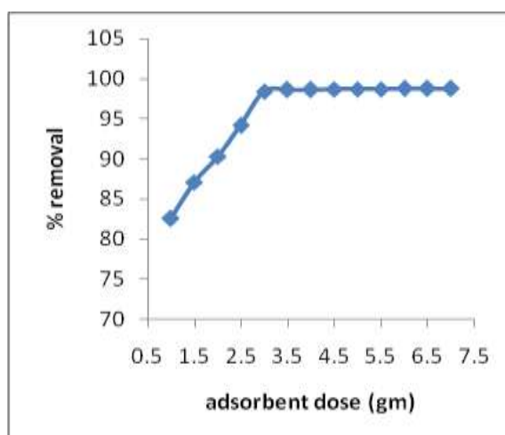
Fig. 10: The removal of Chromium(VI) and plot percent of adsorbent dose function
