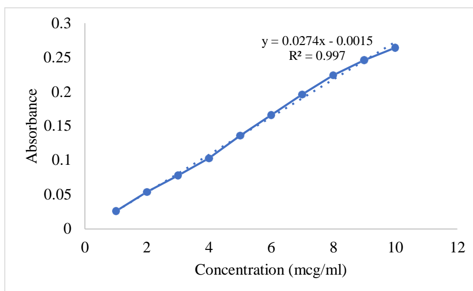
Figure 1: Calibration curve of Losartan potassium drug
