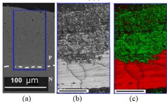
Fig. 8: EBSD ANALYSIS OF PRISMATIC LAYER OF H. RUFESCENS (a) SECONDARY ELECTRON IMAGE, (b) DIFFRACTION INTENSITY MAPS, (c) PHASE MAP
