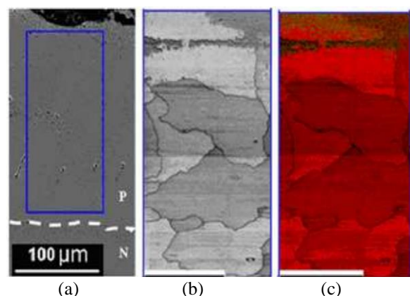
Fig. 8: EBSD ANALYSIS OF PRISMATIC LAYER OF H. RUFESCENS (a) SECONDARY ELECTRON IMAGE, (b) DIFFRACTION INTENSITY MAPS, (c) PHASE MAP
