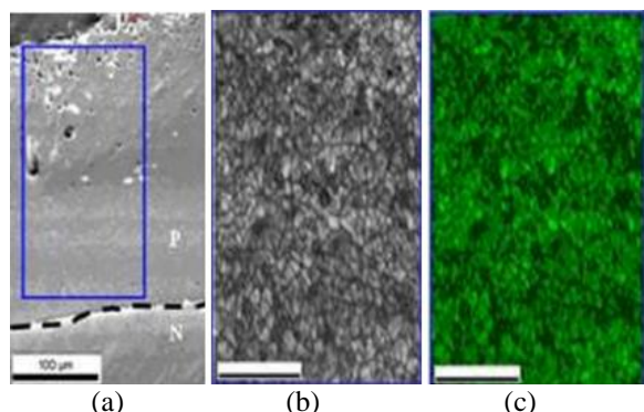
Fig. 7: EBSD ANALYSIS OF PRISMATIC LAYER OF H. ASININE, (a) SECONDARY ELECTRON IMAGE, (b) DIFFRACTION INTENSITY MAPS, (c) PHASE MAP
