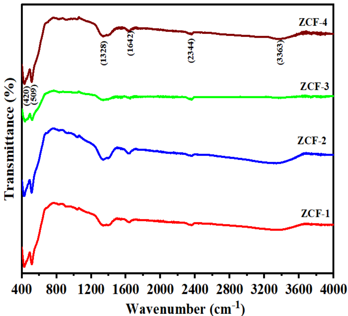
Figure 3: FTIR spectra of \text{Zn}_{1-x}\text{Cu}_x\text{Fe}_2\text{O}_4 ( x=0.2-0.8 ) (ZCF) nanoparticles
