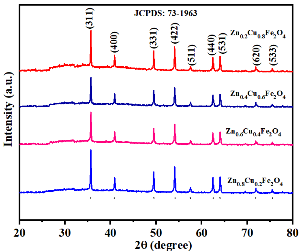
Figure 1: XRD patterns of Zn 1-x Cu x Fe 2 O 4 (x=0.2-0.8) (ZCF) nanoparticles
