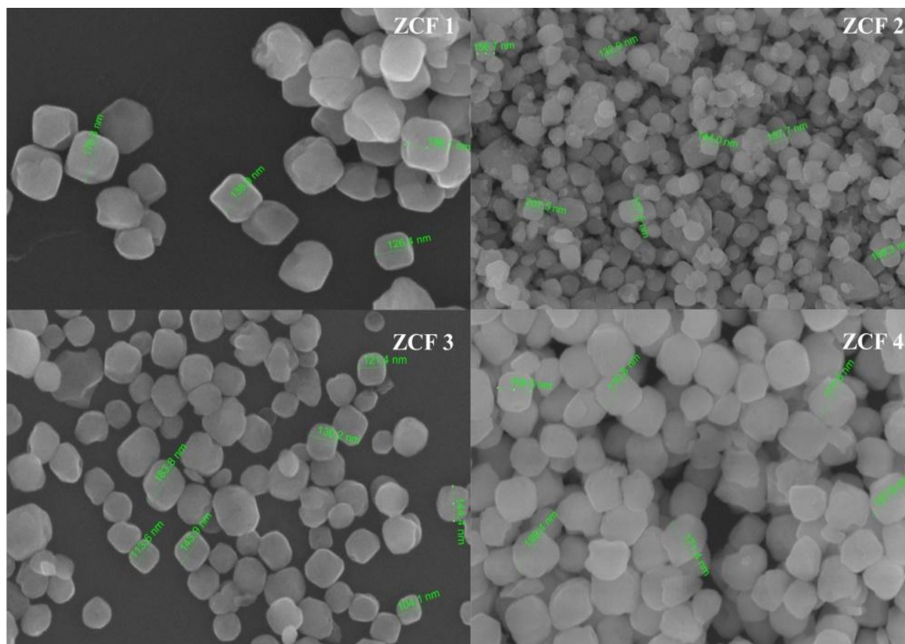
Figure 2: SEM pictures of Zn_{1-x}Cu_xFe_2O_4 ( x=0.2-0.8 ) (ZCF) nanoparticles
