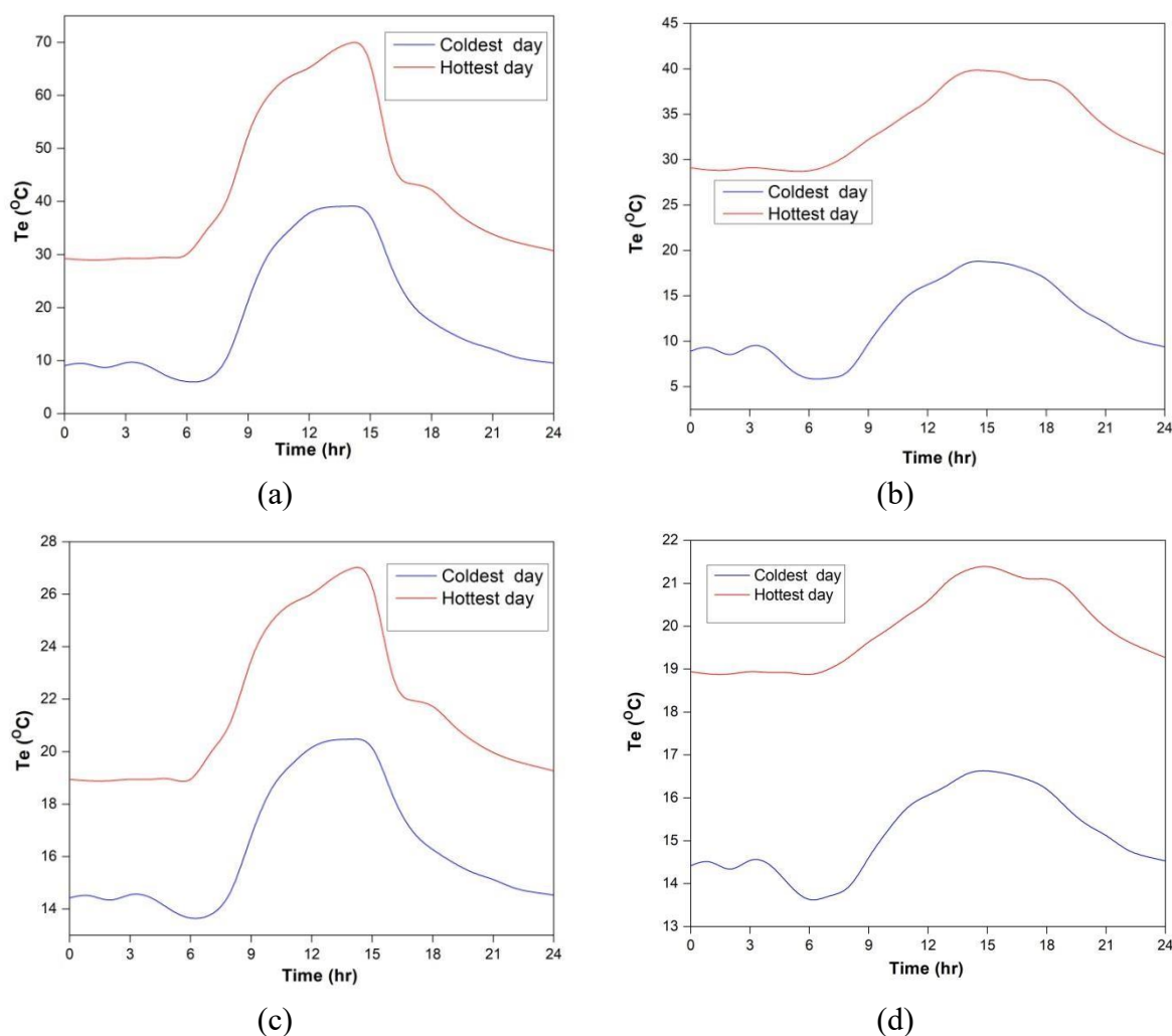
Figure 7. Hottest summer and Coldest winter day T_e fluctuation for (a) dry sunlight surface, (b) dry sheltered surface, (c) wet sunlight surface, and (d) wet sheltered surface
