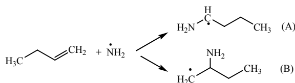
Scheme 1. Amination of 1-butene
